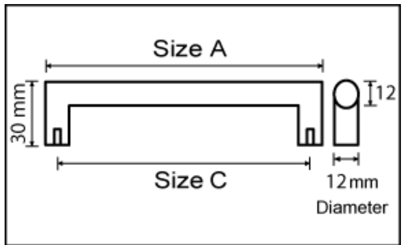
E5023 Stainless Steel Handle
